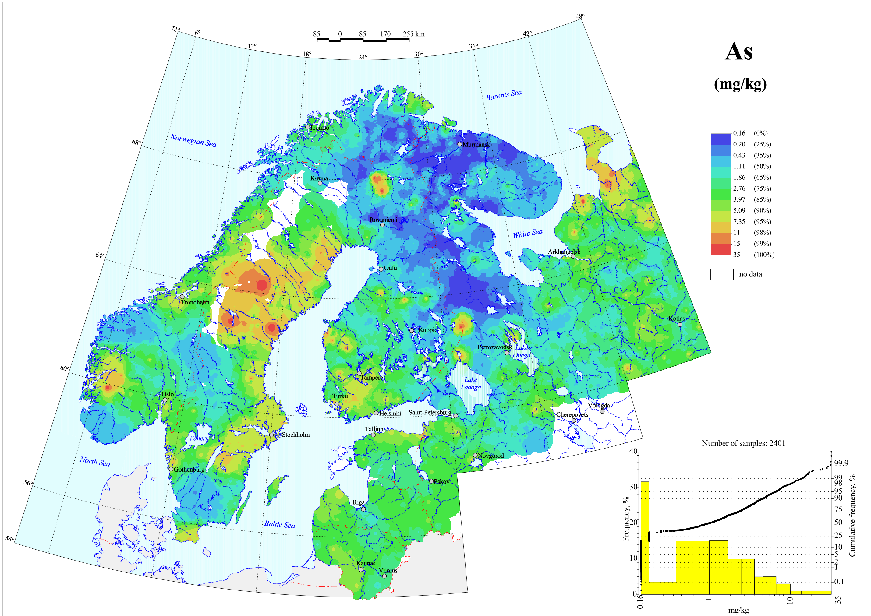
Arsenic in C-horizon, Grain Size <2 mm, Total Content
